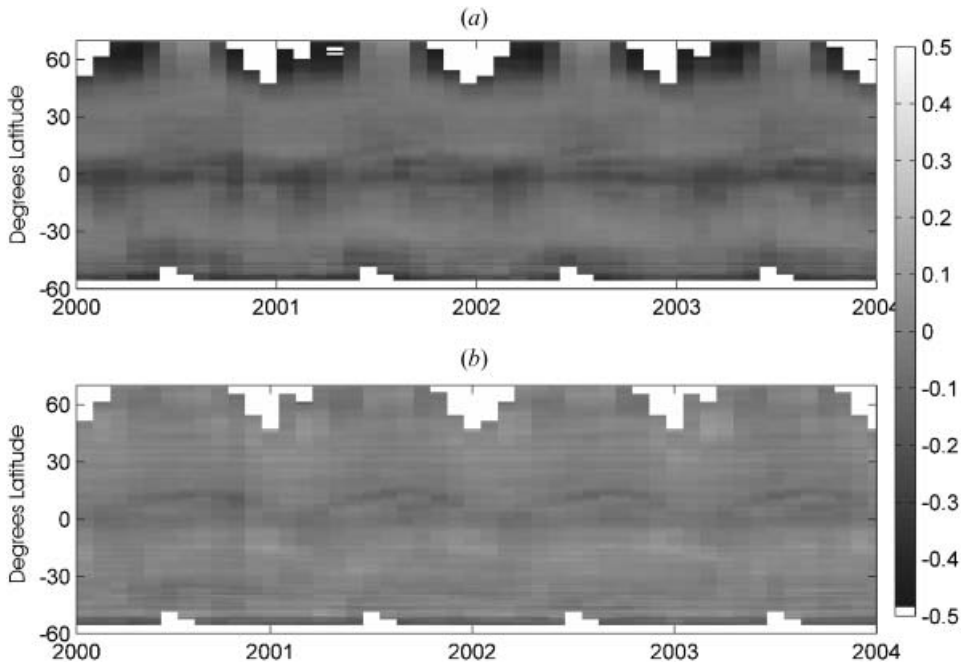
Figure 3. Zonal mean (averaged per latitude) of the difference between MODIS and AVHRR (a) and MODIS and NNdvi (b) through time from 2000 to 2003.
