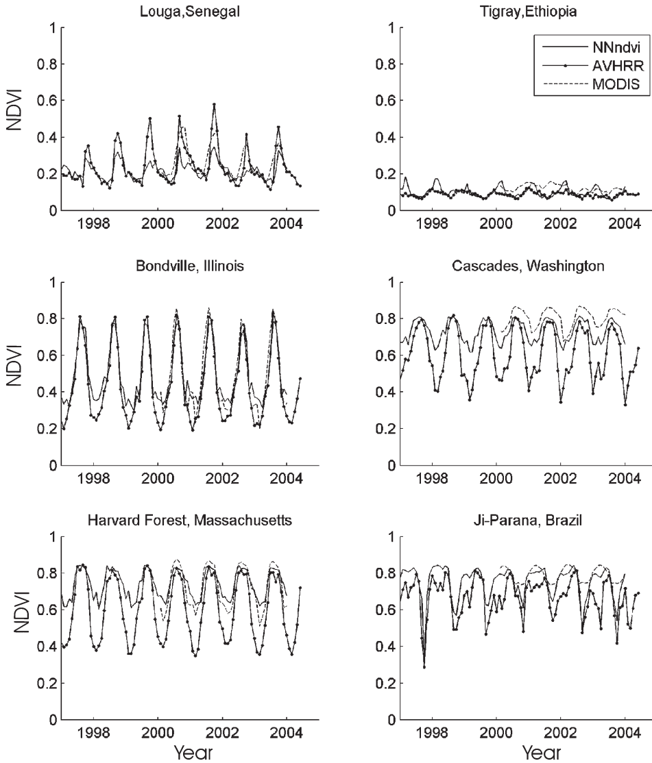
Figure 6. Time series plots of six latitude-longitude locations: Louga, Senegal (16, -16), Tigray Ethiopia (14, 40), Bondville Illinois (10, -88), Cascades Washington (44,-122), Harvard Forest Massachusetts (43, -72), and Ji-Parana Brazil (-11, -62).
